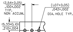
RECOMMENDED P.C. BOARD LAYOUT FOR ASS'Y. PROC. A
