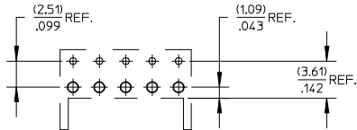
RECOMMENDED P.C. BOARD LAYOUT FOR ASS'Y. PROC. C
